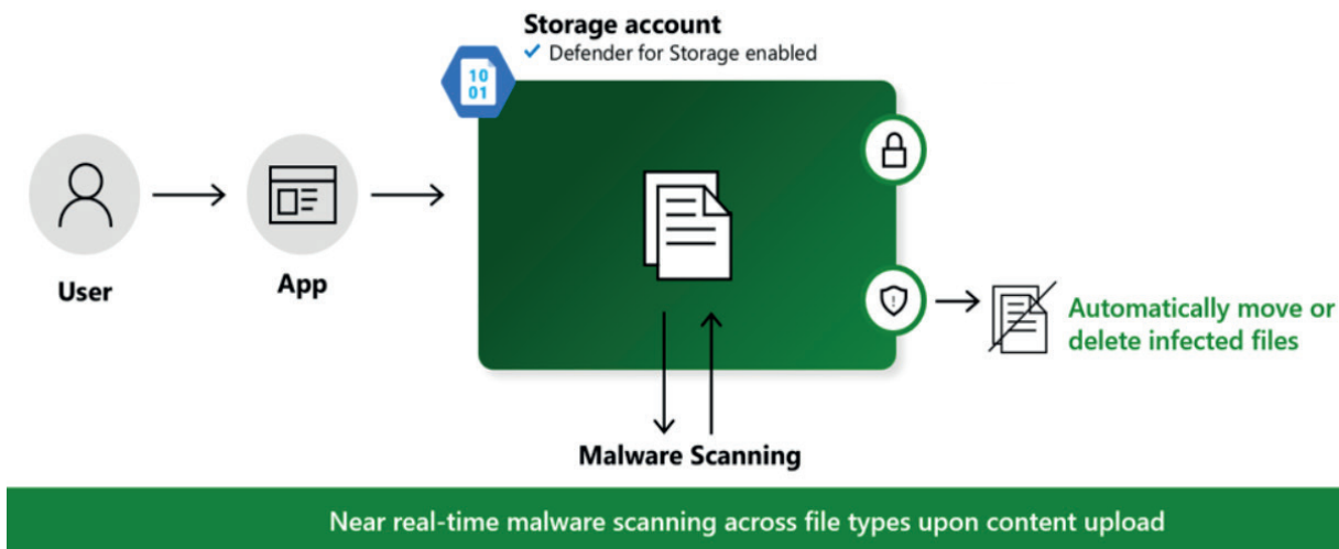
Figure 1: Detect Malicious Files Upon Upload in Near Real Time for Azure Blob Storage For more information, visit learn.microsoft.com/en-us/azure/defender-for-cloud
